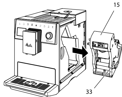
Fig. 14: Removing the brewing unit
